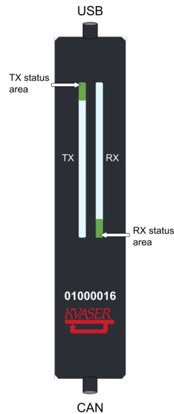
Figure 5: The TX and RX LED bars on the Kvaser U100-X3 includes status areas.
