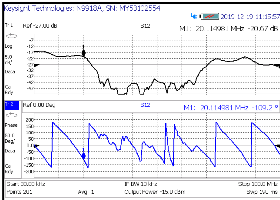
Figure 9: The S12 parameters from the source at 16 to receiver at 17 (with figure 8 CAN-bus layout) for all frequencies from 0 to 100 MHz. Upper graph shows loss in dB; lower shows phase shift.
