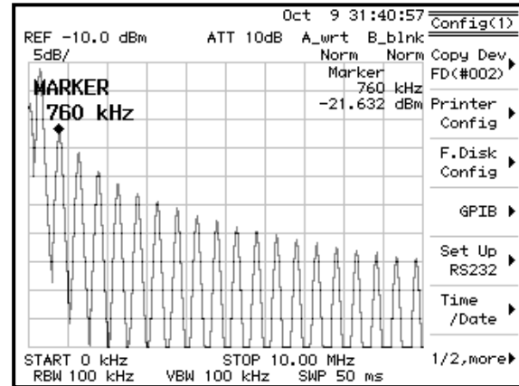
Figure 13: Spectrum for a square wave at 250 kHz with a 5 ns slew-rate.
