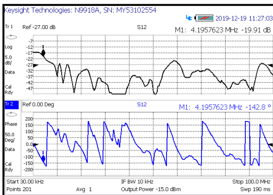
Figure 10: S12 from source at 16 to receiver at 17 from 0 to 100 MHz with CAN-bus as shown in figure 6.
