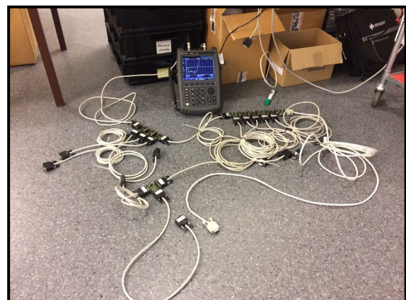
Figure 3: Shows the TDR measurement, with all drop lines installed.
