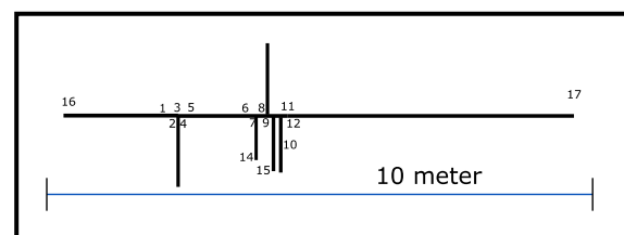
Figure 8: A 9.6-meter CAN-bus with 5 short drop lines.
