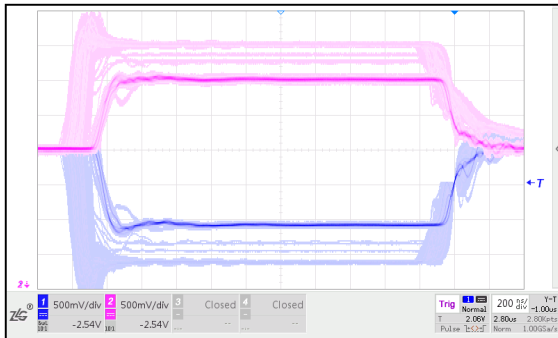
Figure 21: Dominant signal at connection 17 at 0.5 Mbit/s with oscilloscope in persist mode.
