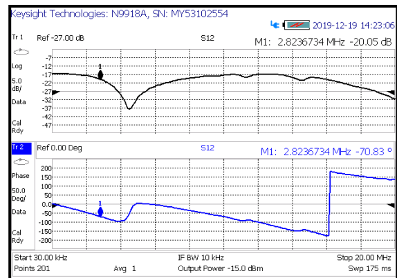
Figure 12: S12 from 16 to end of segment 2, frequency range 0 to 20 MHz.
