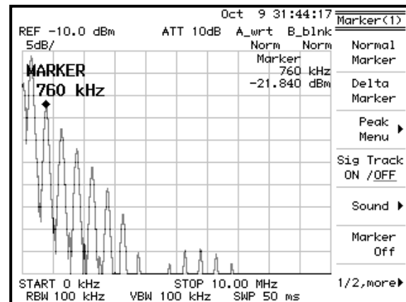
Figure 14: Spectrum for a square wave at 250 kHz with a 200 ns slew-rate.
