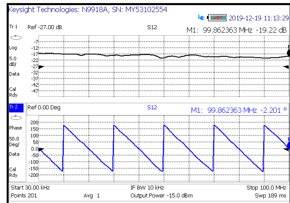
Figure 7: S12 from source at 16 to receiver at 17, from 0 to 100 MHz with CAN-bus layout as shown in figure 1.
