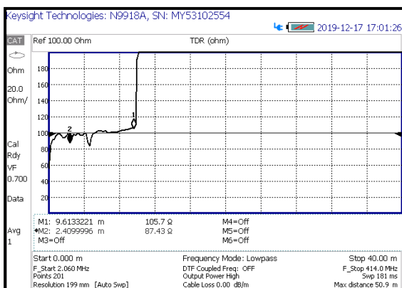
Figure 1: A 9.6 meter long cable.
