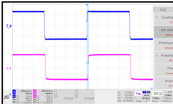
Figure 15: Top signal at connection 16 and lower signal at connection 17, in figure 1. 250 kHz with 5 ns slew-rate.
