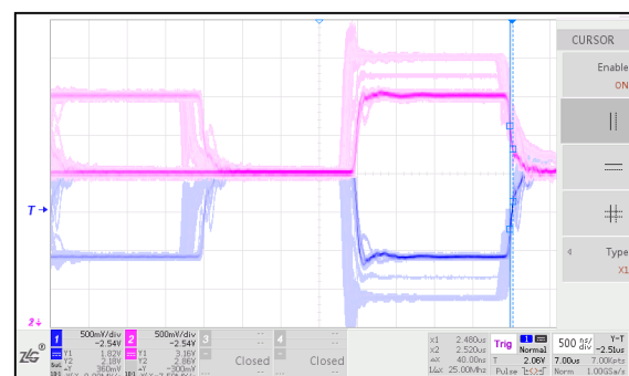
Figure 20: Dominant signal at connection 17 at 1 Mbit/s with oscilloscope in persist mode.
